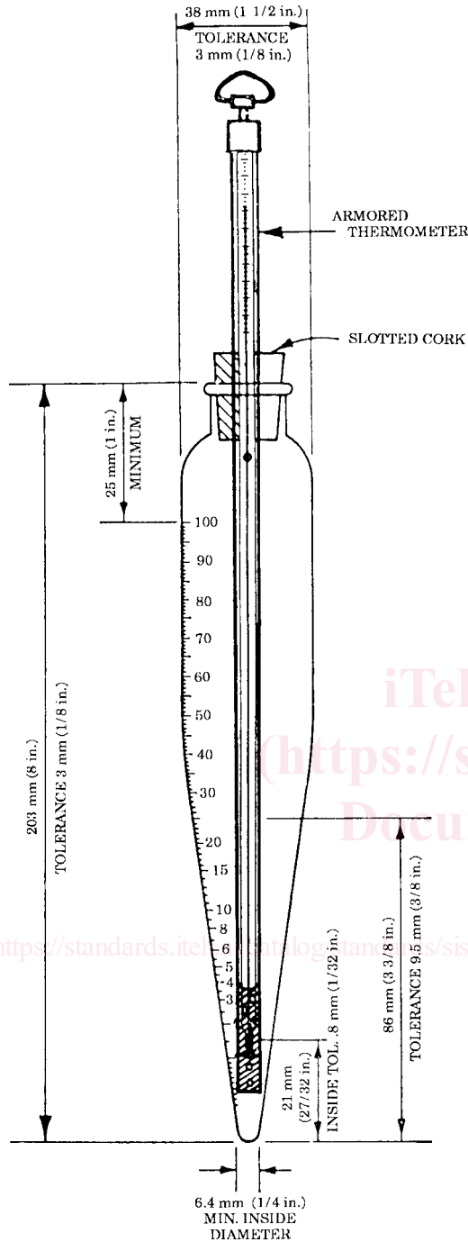
NOTE 1—For graduation tolerances see Table 1. FIG. 1 Weathering Tube
