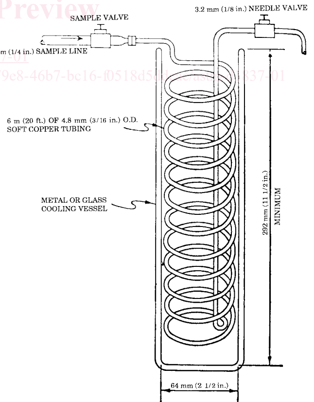
NOTE 1—The coils in the drawing are extended for clarity. FIG. 2 Precooling Equipment
