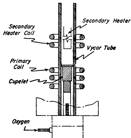
FIG. 1 Combustion Tube
