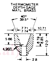
GREASE CUP MATL. CHROMIUM PLATED BRASS
