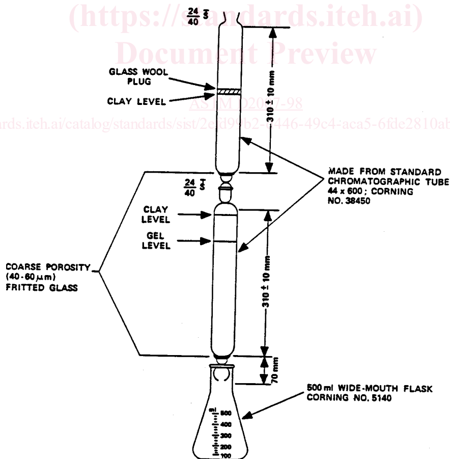
FIG. 1 Clay-Gel Percolating Column
