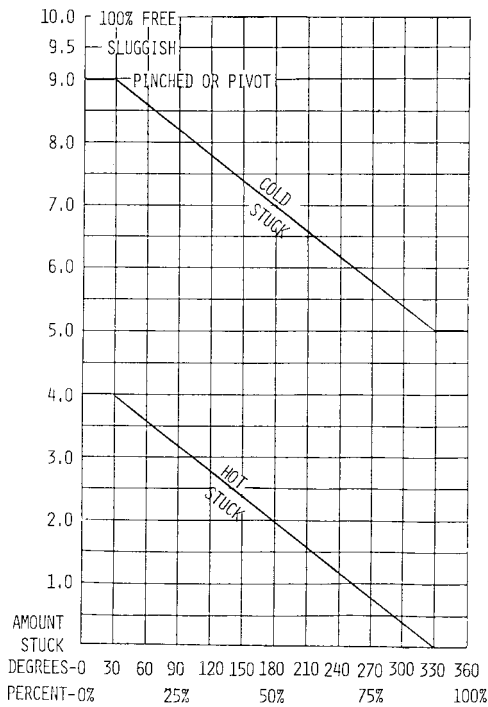
FIG. 2 Ring Sticking Rating Chart
