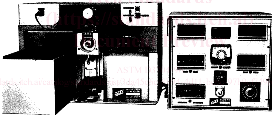
FIG. 1 Falex Ring and Block Test Machine (continued)
