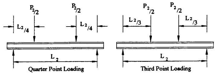
FIG. 2 Two-Point Load
