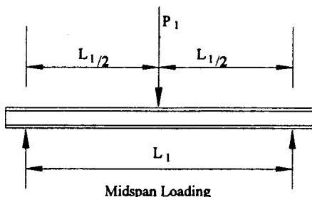
FIG. 1 Single-Point Load
