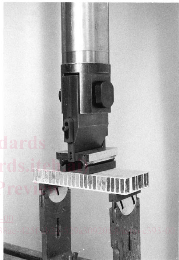
FIG. 3 Short Beam—Two-Point Load (Third Point)
