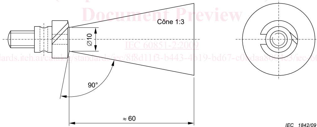
Figure 1 – Conical mandrel
