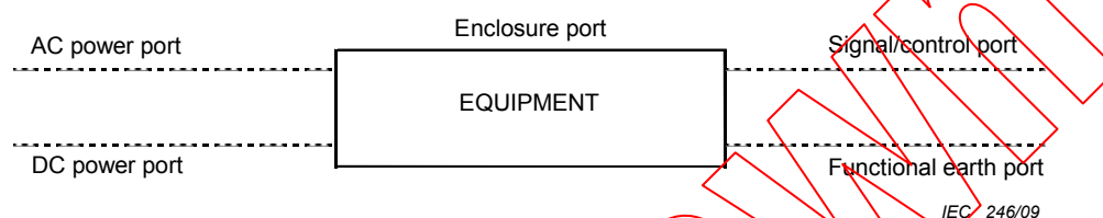
Figure 1 – Equipment ports
