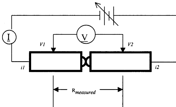
FIG. 1 Schematic Representation of 4 Wire Measurement Circuit
