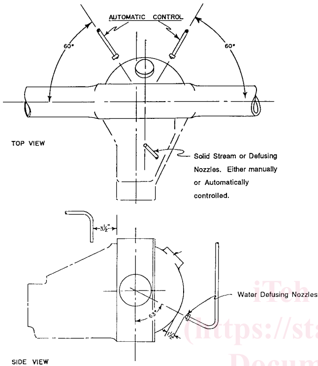
NOTE 1—Use 3/8 in. tubing for all water lines. FIG. A5.1 Location of Spray Nozzles on Axle
