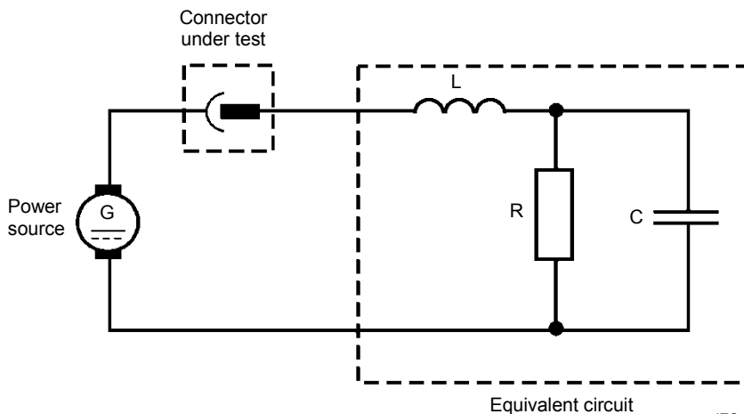
Figure A.2 – Example of circuit(s) – Circuit diagram
