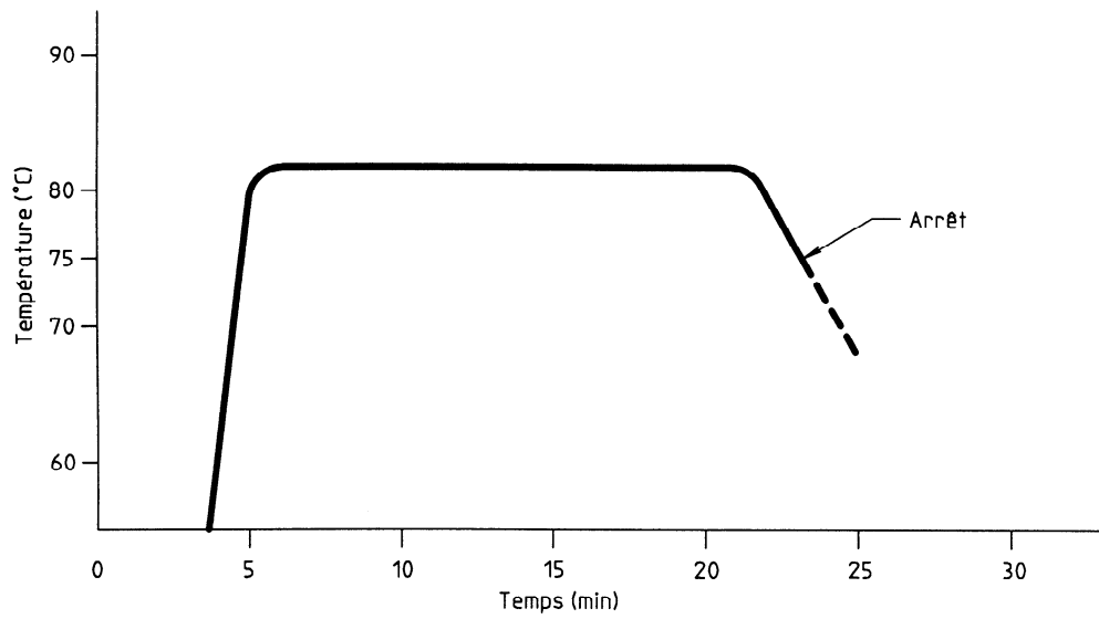
Figure 2 — Courbe de distillation type
