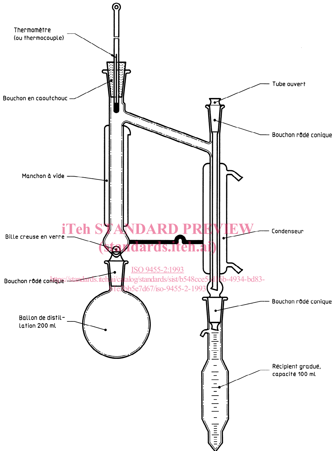
Figure 1 — bulliomtre Martin  ballon de distillation sphrique
