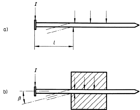
Figure 4 — Principle of the three-point impact method by impact load (impulse) I , showing angle of deformation \beta
