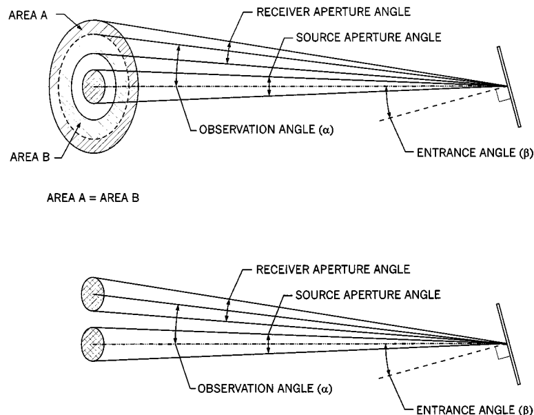
FIG. 1 Annular and Point Aperture Instrument Angles
