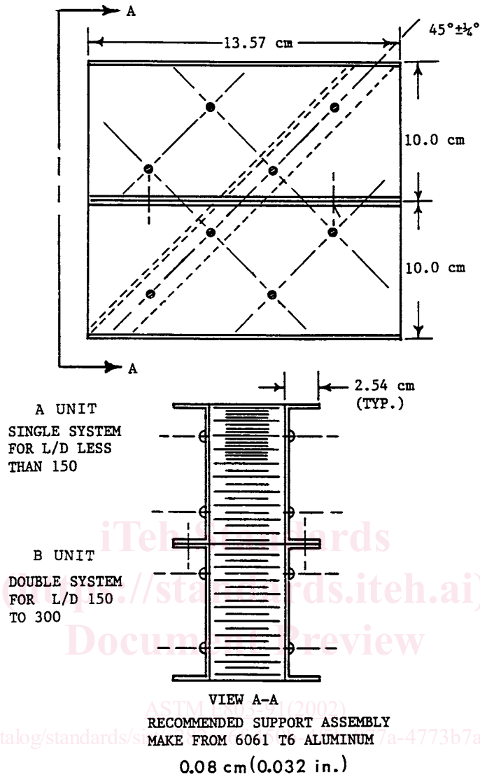
2(b) L/D Apparatus Assembly
