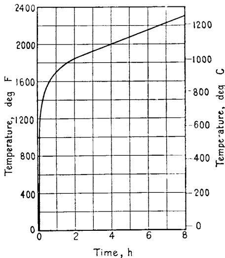
FIG. 1 Temperature-Time Curve
