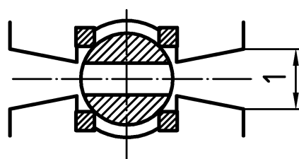
Figure 1b — Reduced bore
