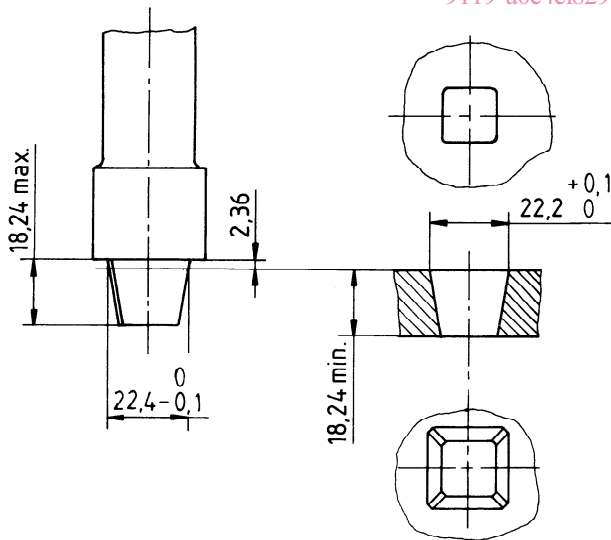
a) Clearance to shoulder
