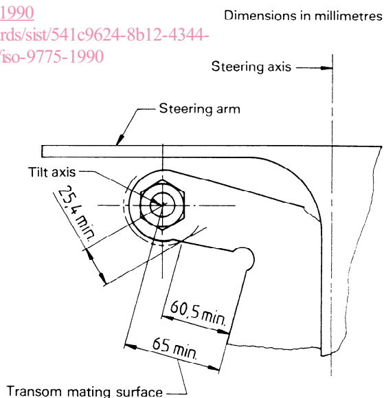
Figure 4 — Motor-mounted steering tilt axis
