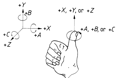
Figure 2 — Rotary motions
