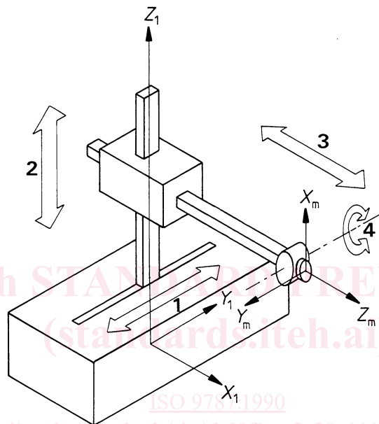
Figure A.1 — Rectangular robot
