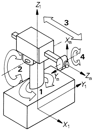
Figure A.3 — Polar robot
