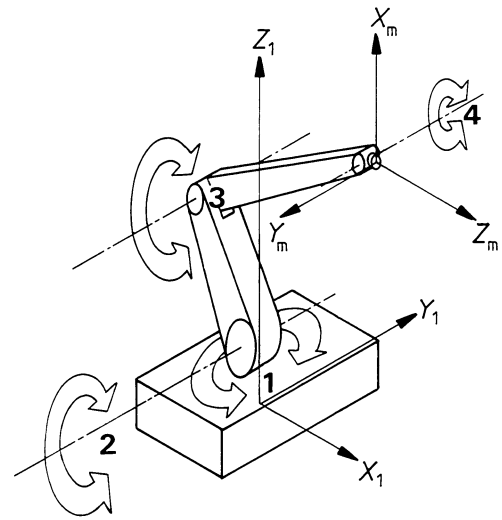
Figure A.4 — Revolute robot
