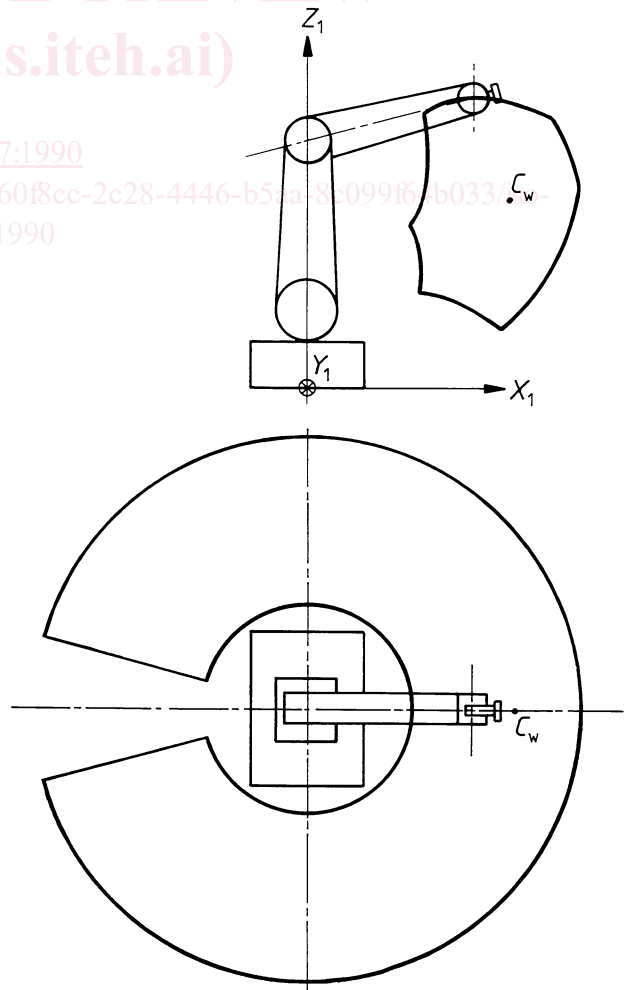
Figure 4 — Example of robot working space
