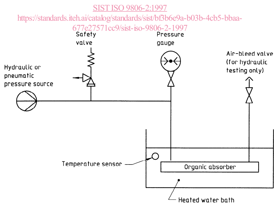
Figure 2 — Schematic for internal pressure test of organic absorbers for use in unglazed collectors
