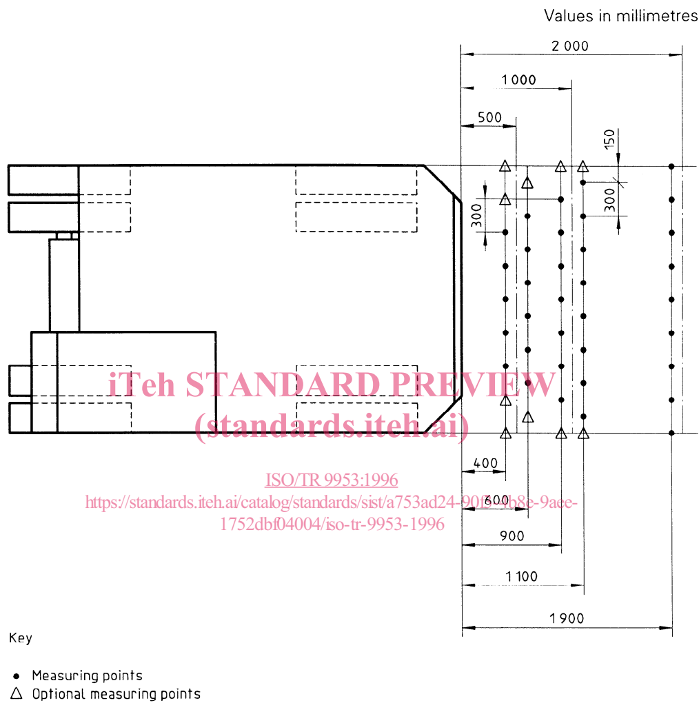
Figure 2 — Horizontal warning range and test grid for static test
