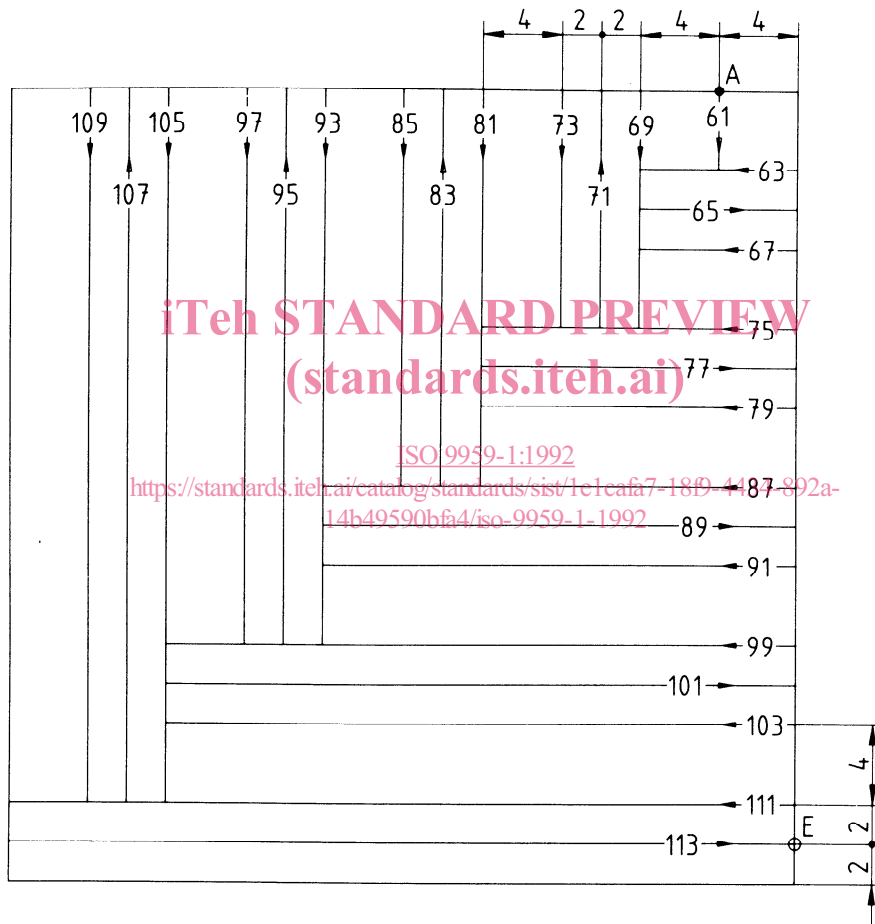
Figure 5 — Parallel lines: zone 3
