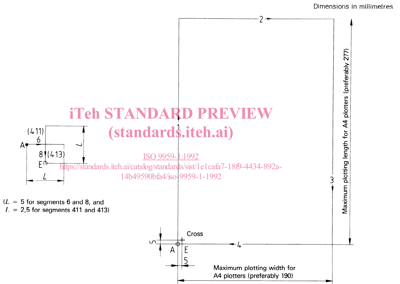
Figure 2 — Border line/cross marks: zone 0
