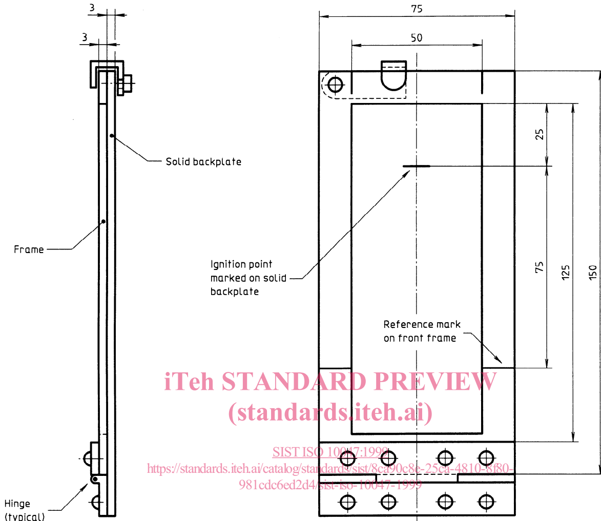
Figure 1 — Specimen holder
