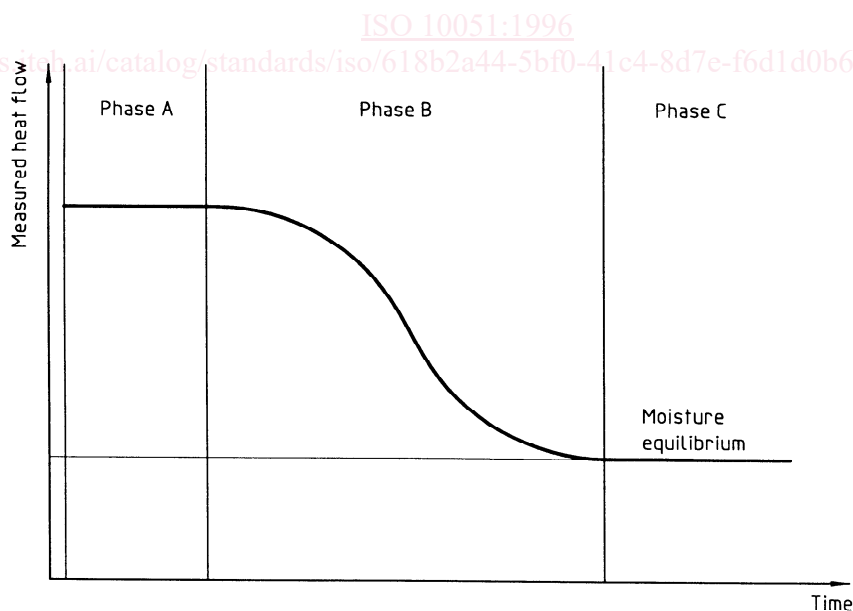
Figure 1 — Heat flow during a test to determine thermal transmissivity of a moist material
