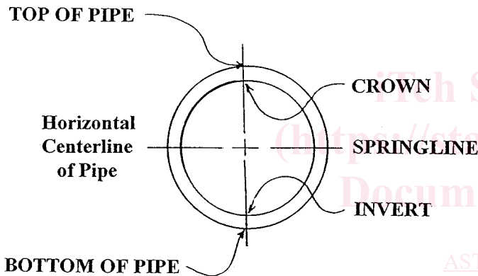
FIG. 2 Pipe Terminology
