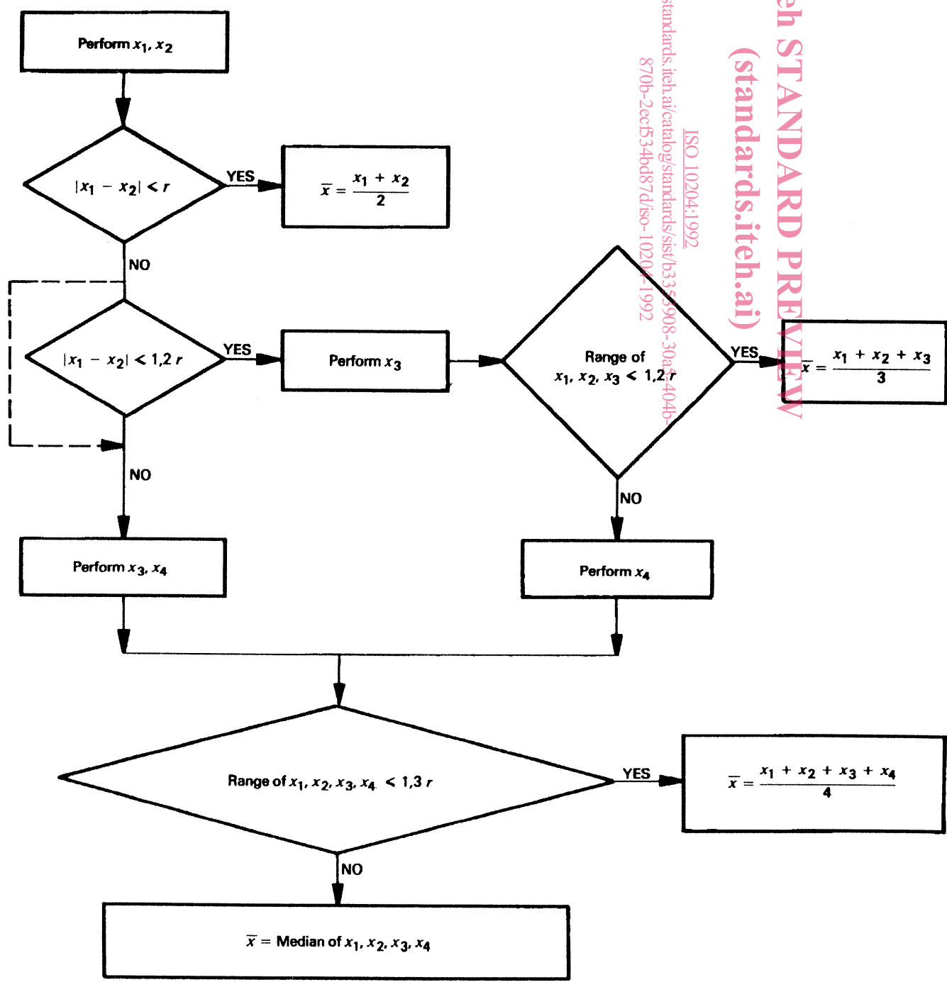
Flowsheet of the procedure for the acceptance of analytical values for test samples
