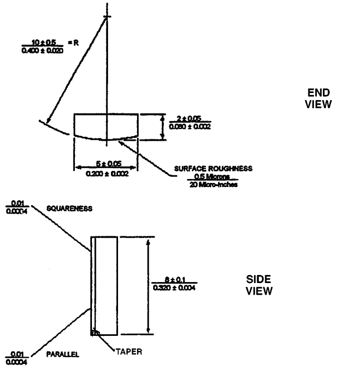
NOTE 1—Top number denotes millimetres: lower number denotes decimals of an inch. FIG. 6 Load Contact Surface – Sapphire (Synthetic)
