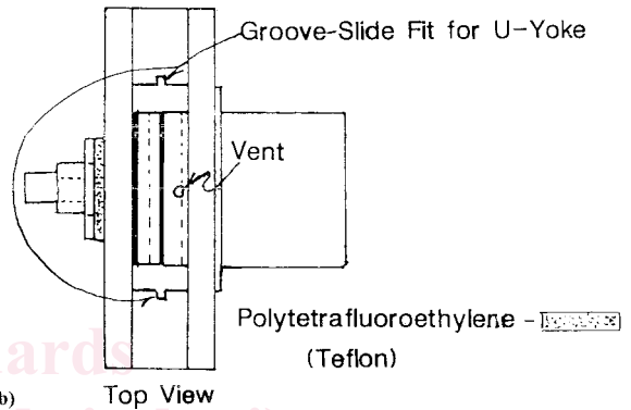
FIG. 2 Cell for Test Method B
