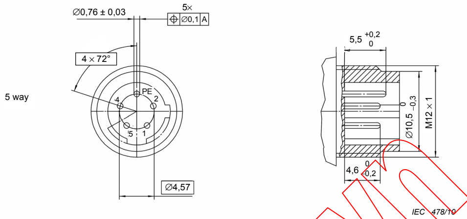
Figure 27 – Pin front view 5 way with C-coding
