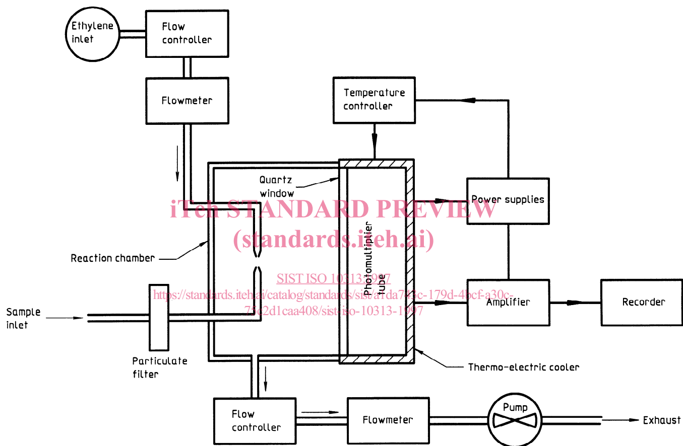
Figure 1 — Schematic diagram of a chemiluminescence ozone analyser
