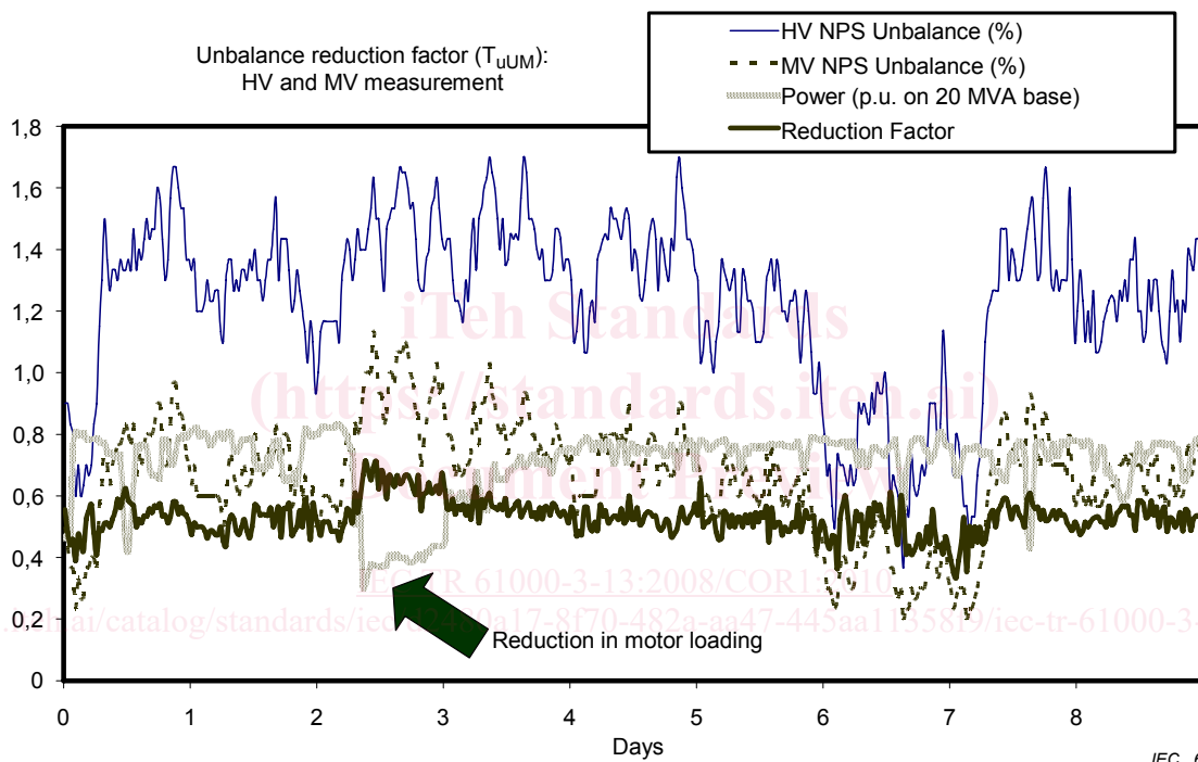
Figure A.2 – Example of unbalance ratio measurement for a remote mine with largely motor loading
