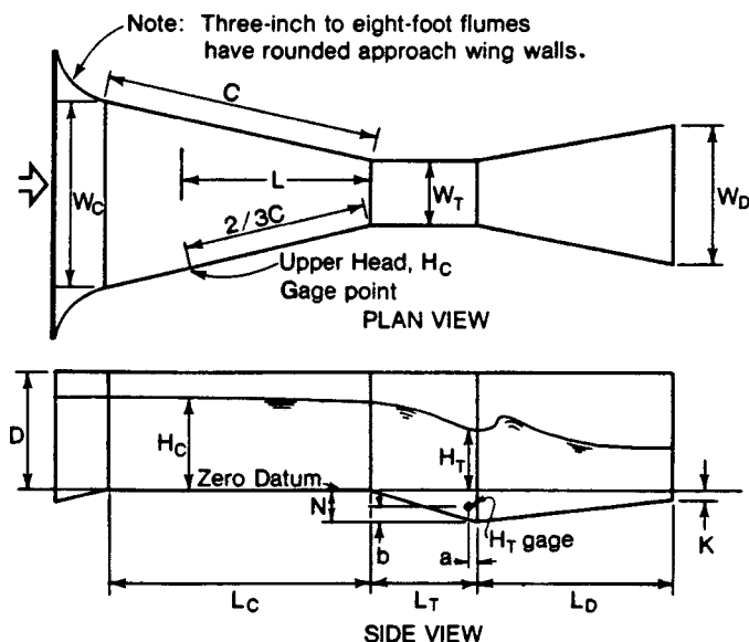
FIG. 1 Parshall Flume
