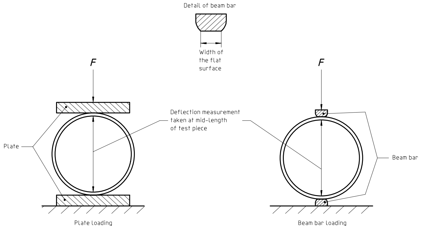
Figure 1 – Schematic diagram of the test arrangement (standards.iteh.ai)
