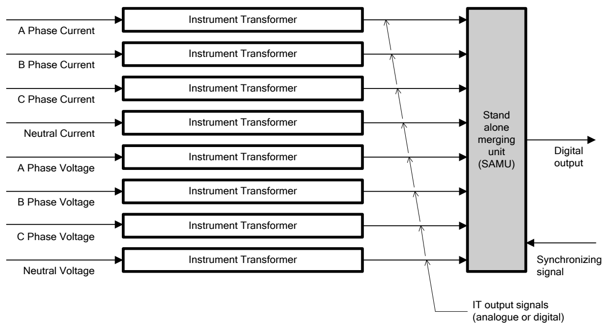
Figure 904 – Standalone merging unit
