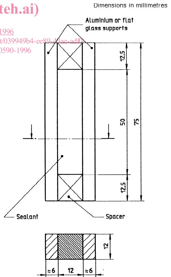
Figure 2 — Test specimen with aluminium or flat glass supports
