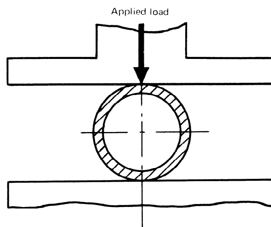
FIGURE 2 – Test arrangement
