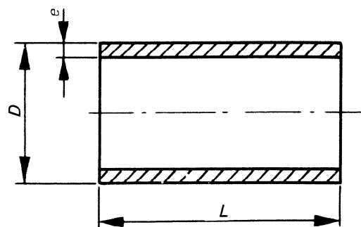
FIGURE 1 – Test piece
