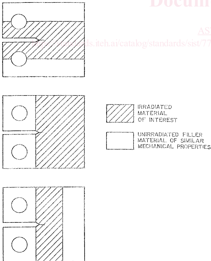
FIG. 2 Various Forms of End-Tab Welded (Compound) Specimens
