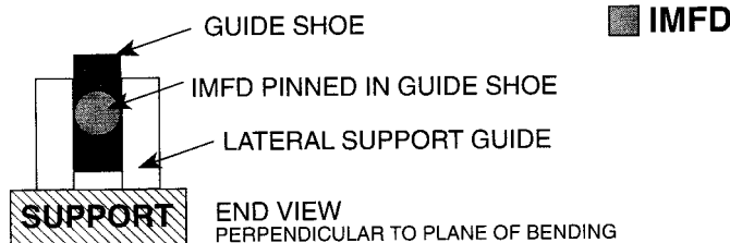
FIG. A1.2 4-Point Bend Test with Guide Shoes
