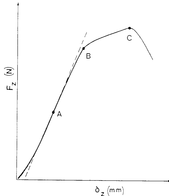
NOTE 1—Stiffness is defined as the slope of the linear-most portion of the curve, here evaluated by a tangent drawn at Point A. Point B illustrates a slope discontinuity (possibly indicative of interfacial slip or subcomponent failure within the connector), and Point C illustrates the maximal load acceptance (ultimate strength).
