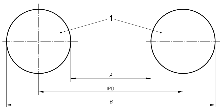
Figure 1 — Test configuration for measuring the interpupillary distance
