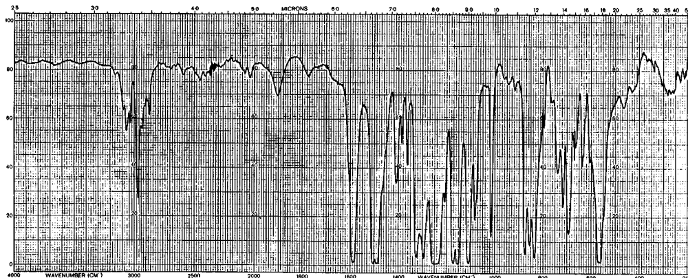
FIG. 1 Polysulfone Infrared Spectrum—Percent Transmittance for 0.0005 in. Film
