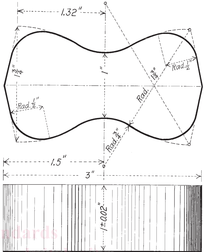
FIG. 2 Briquet Specimen for Tensile Strength Test
