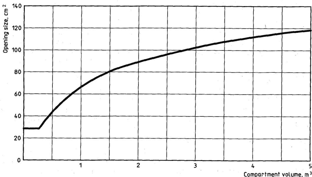
Figure 1 — Natural ventilation opening size
