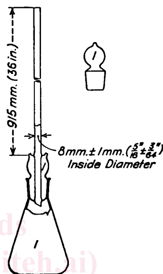
FIG. 1 Apparatus for Determination of Organically Combined Sulfuric Anhydride, Test Method A
