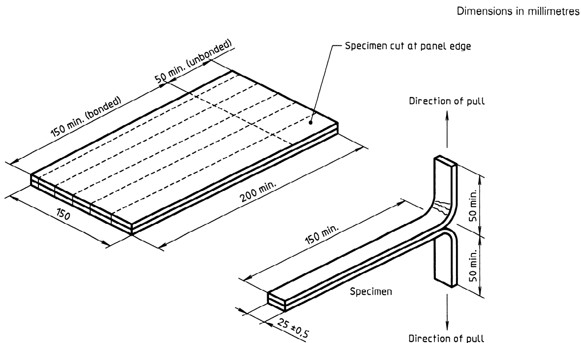
Figure 1 — Panel before cutting and individual specimen after cutting
