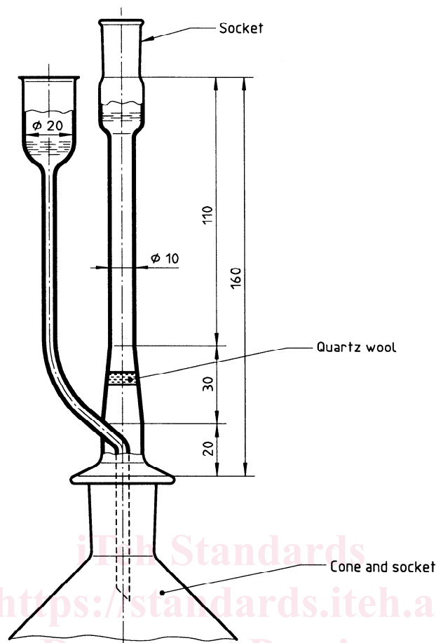
Figure 1 — Microseparator
