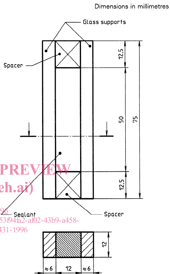
Figure 1 — Assembly for test and reference specimens
