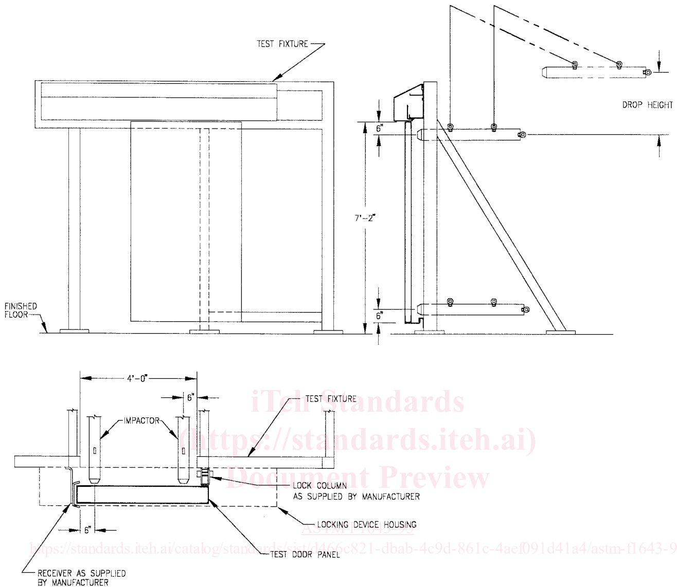
FIG. 1 Test Assembly
