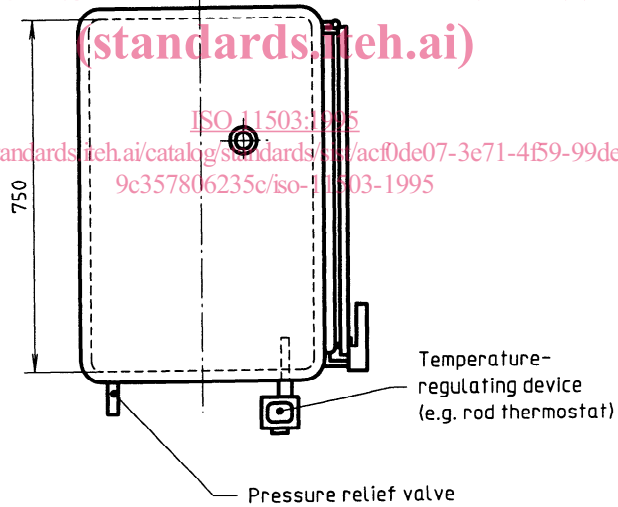
Figure 1 — Airtight cabinet with door
